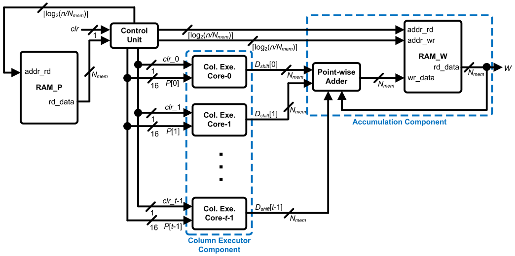
Fig. 4. Overview of the proposed Accelerator-I. Col. Ex.: Column Executor. Notions follow Algorithm 3 and Table 1. addr: address; rd: read; wr: write. N_{mem} : processing bit-length of the memory.
